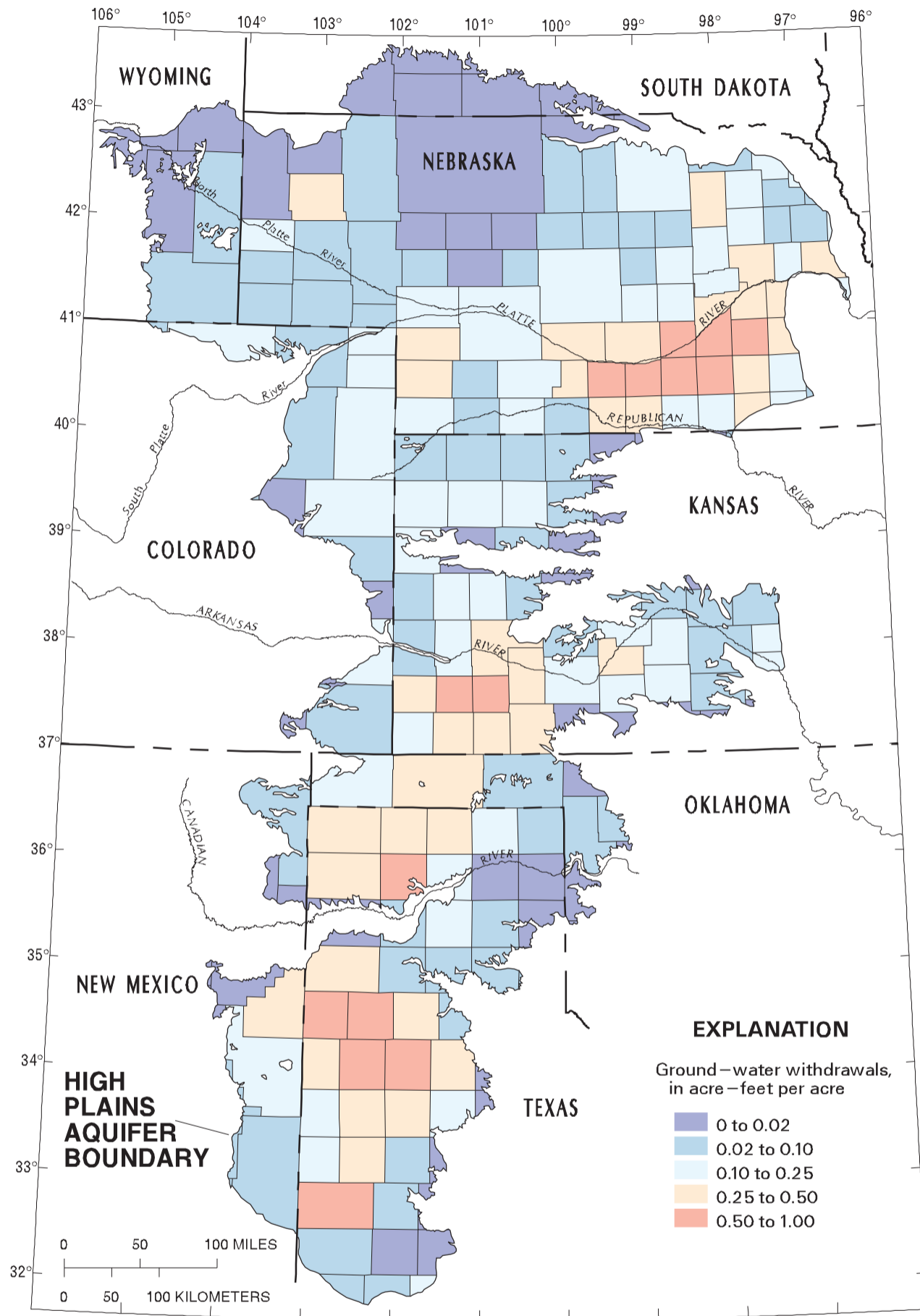
Figure 4. Fresh ground-water withdrawal rates by county during 1995 (data from U.S. Geological Survey Aggregate Water-Use Data System, data retrieved April 1998).
