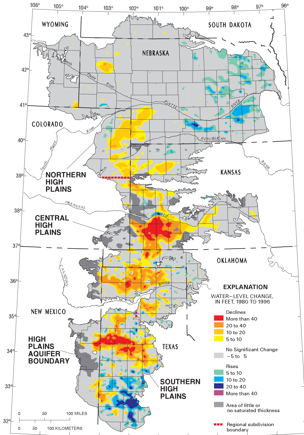
Figure 1. Water-level changes in the High Plains aquifer, 1980 to 1996.
