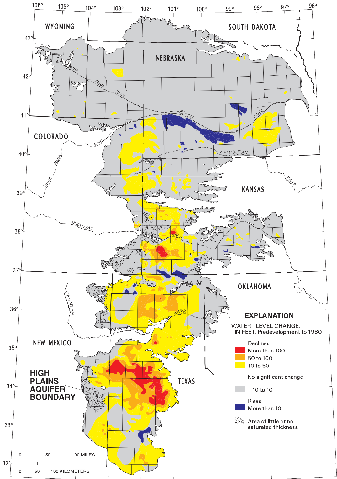
FIGURE 2. Water-level changes in the High Plains aquifer, predevelopment to 1980 (Lucky and others, 1981).
